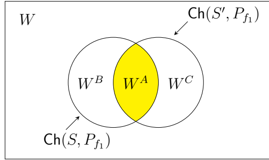
Figure 2: The partition \{W^A, W^B, W^C\} of the workers in \text{Ch}(S, P_{f_1}) \cup \text{Ch}(S', P_{f_1}) .
